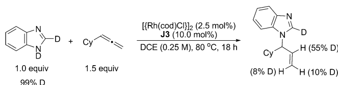
Scheme 2. Isotope-labeling experiments with [\text{D}_2] benzimidazole.
